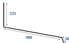
Junction Flashing
